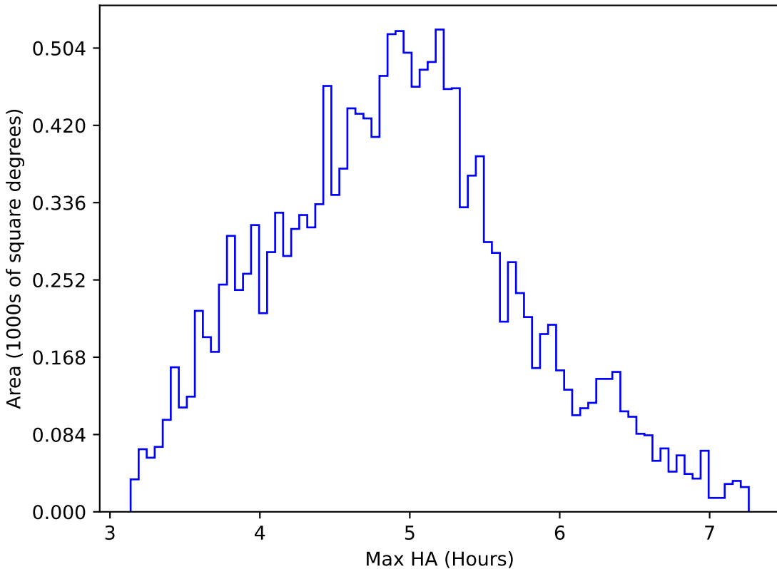
too_elab_r256_d3_griz_v3.4_10yrs WFD i band: Max HA
