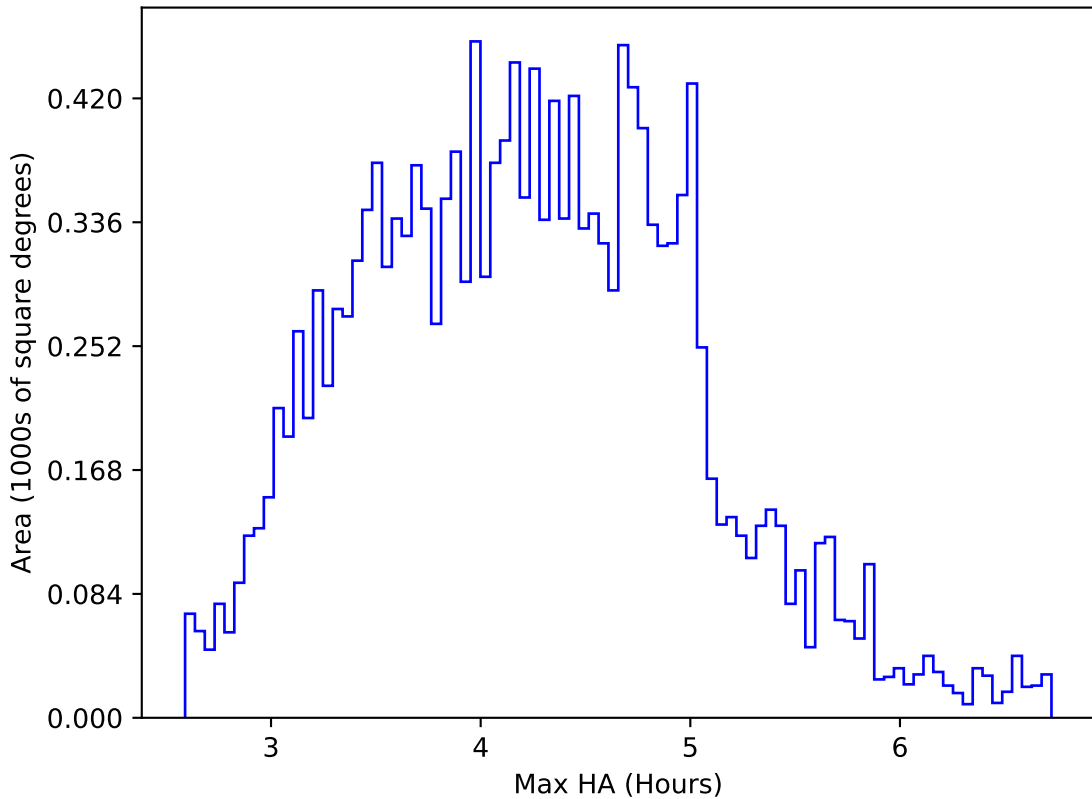
too_elab_r256_d3_griz_v3.4_10yrs WFD g band: Max HA
