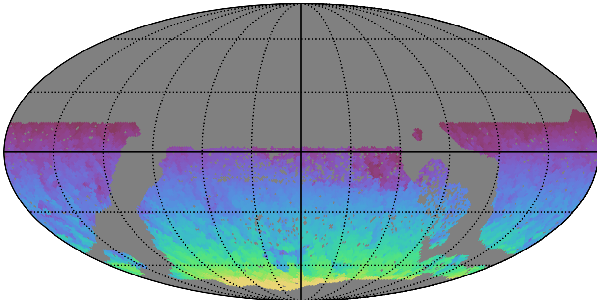
too_elab_r256_d3_griz_v3.4_10yrs WFD all bands: Max HA
