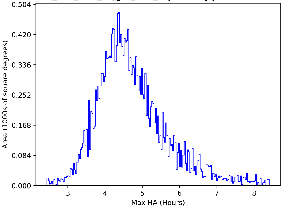
too_elab_r256_d3_griz_v3.4_10yrs All sky y band: Max HA
