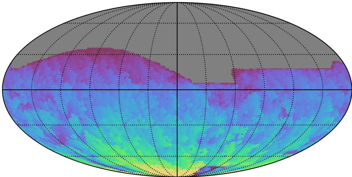
too_elab_r256_d3_griz_v3.4_10yrs All sky r band: Max HA
