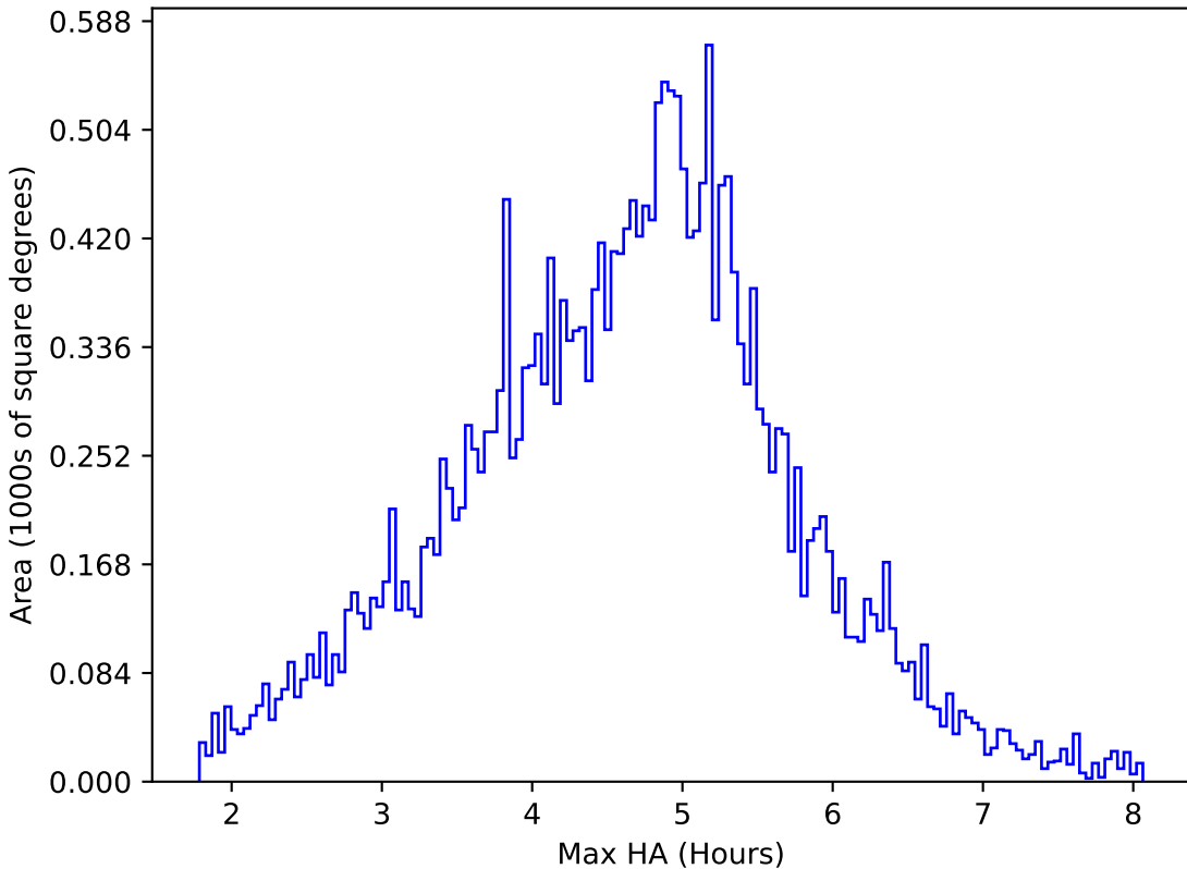
too_elab_r256_d3_griz_v3.4_10yrs All sky i band: Max HA
