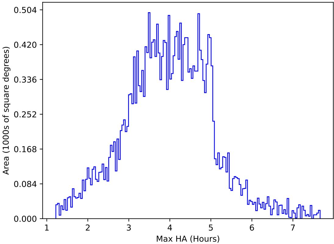
too_elab_r256_d3_griz_v3.4_10yrs All sky g band: Max HA
