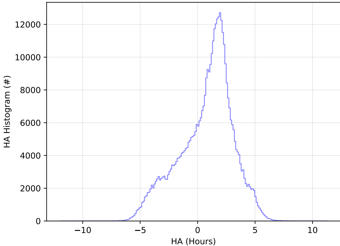
too_elab_r256_d3_griz_v3.4_10yrs WFD z band: HA Histogram
