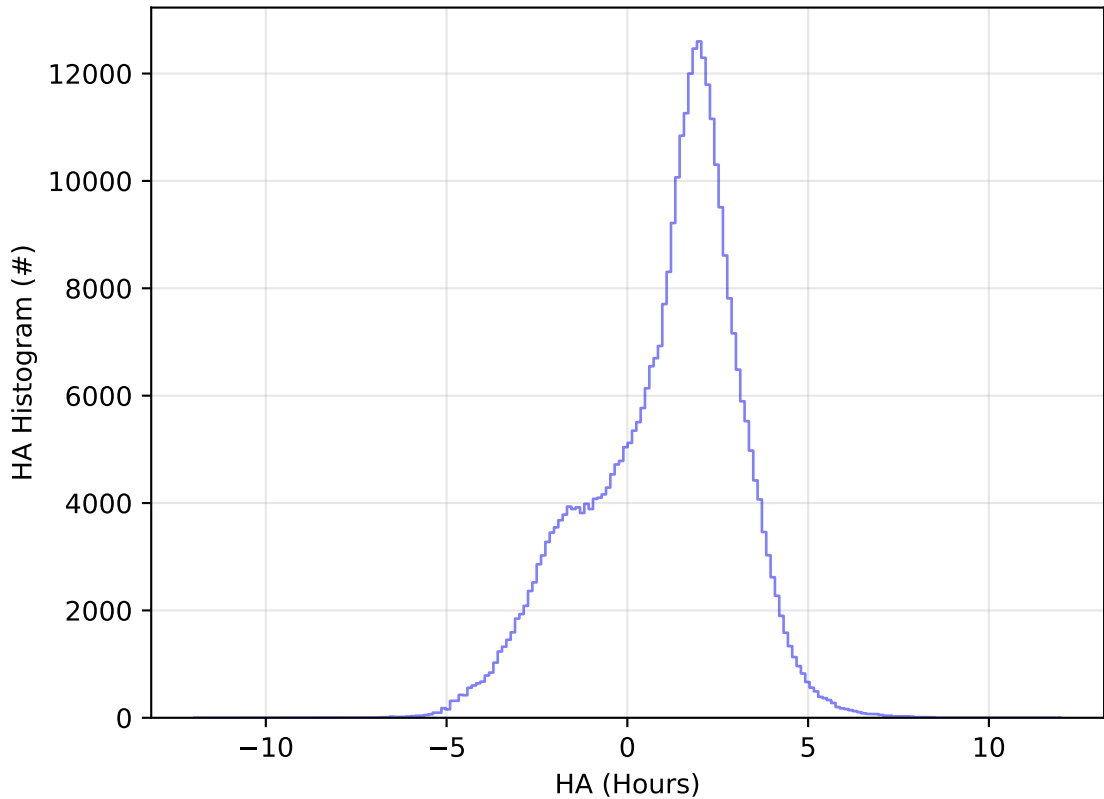
too_elab_r256_d3_griz_v3.4_10yrs WFD y band: HA Histogram
