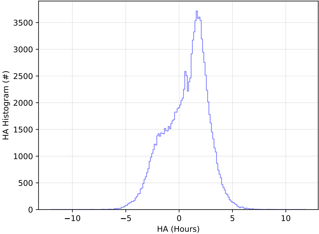
too_elab_r256_d3_griz_v3.4_10yrs WFD u band: HA Histogram
