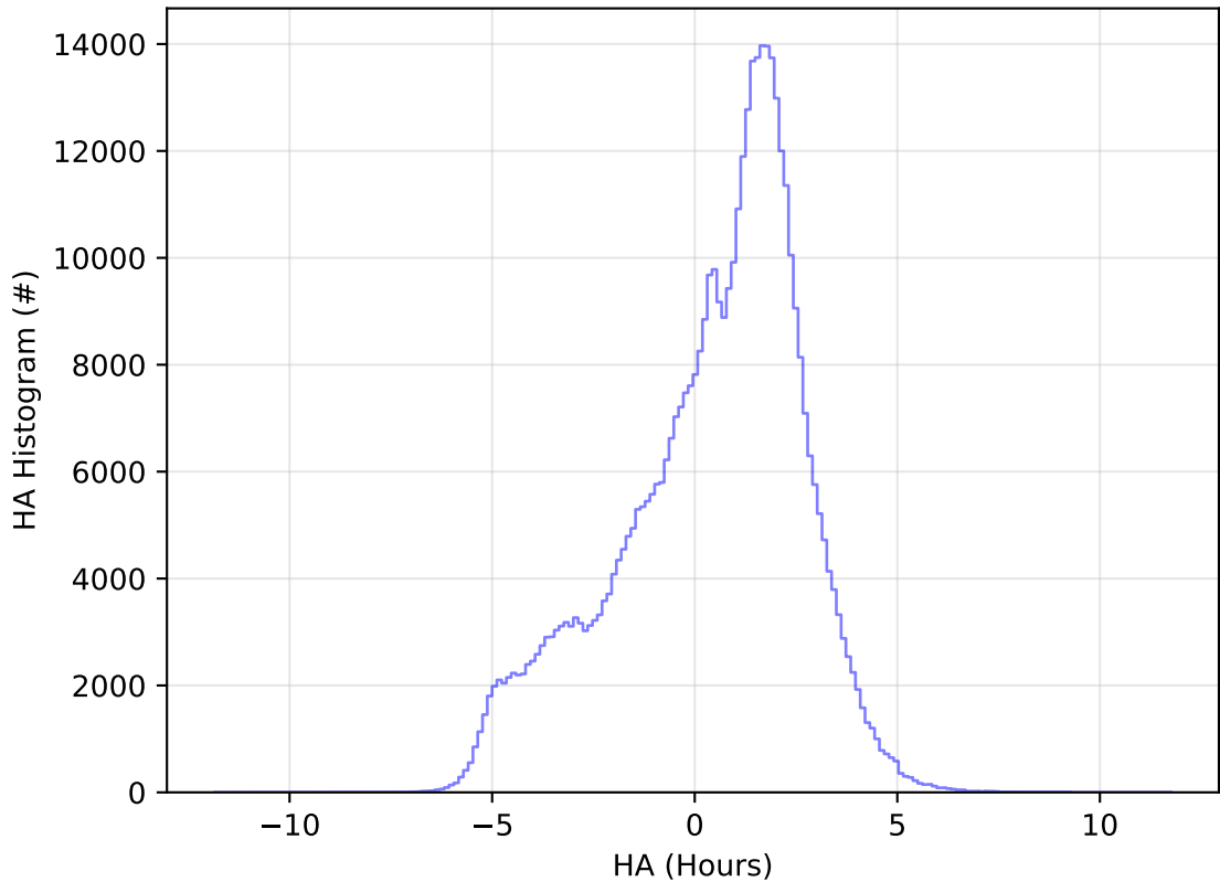
too_elab_r256_d3_griz_v3.4_10yrs WFD r band: HA Histogram
