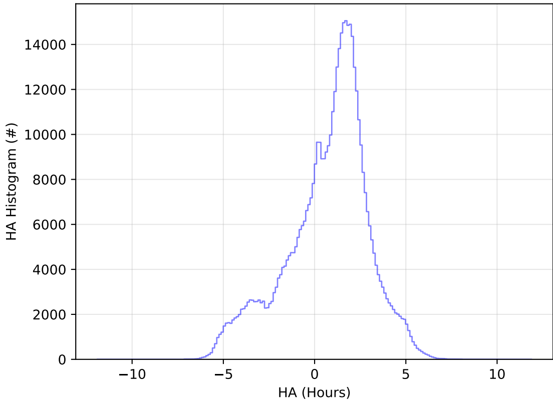
too_elab_r256_d3_griz_v3.4_10yrs WFD i band: HA Histogram
