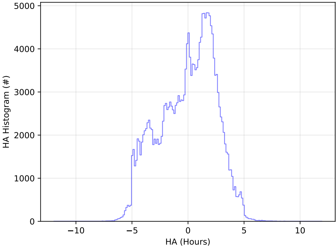
too_elab_r256_d3_griz_v3.4_10yrs WFD g band: HA Histogram
