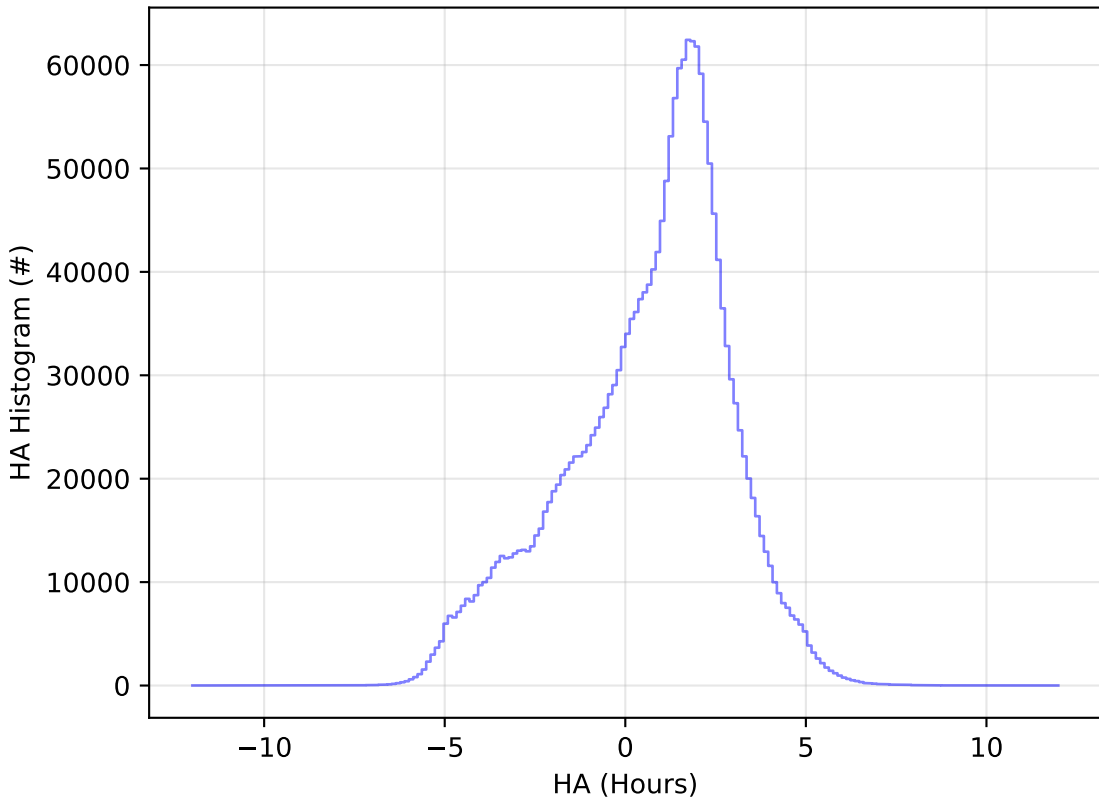
too_elab_r256_d3_griz_v3.4_10yrs WFD all bands: HA Histogram
