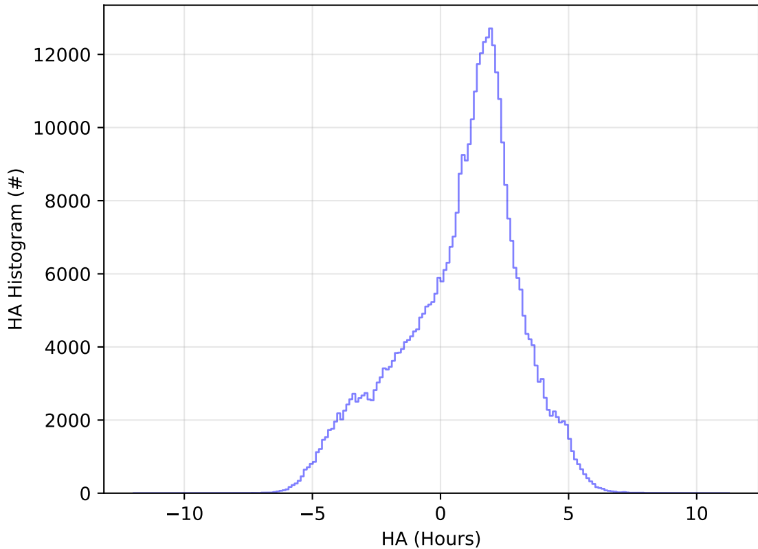
too_elab_r256_d3_griz_v3.4_10yrs All sky z band: HA Histogram
