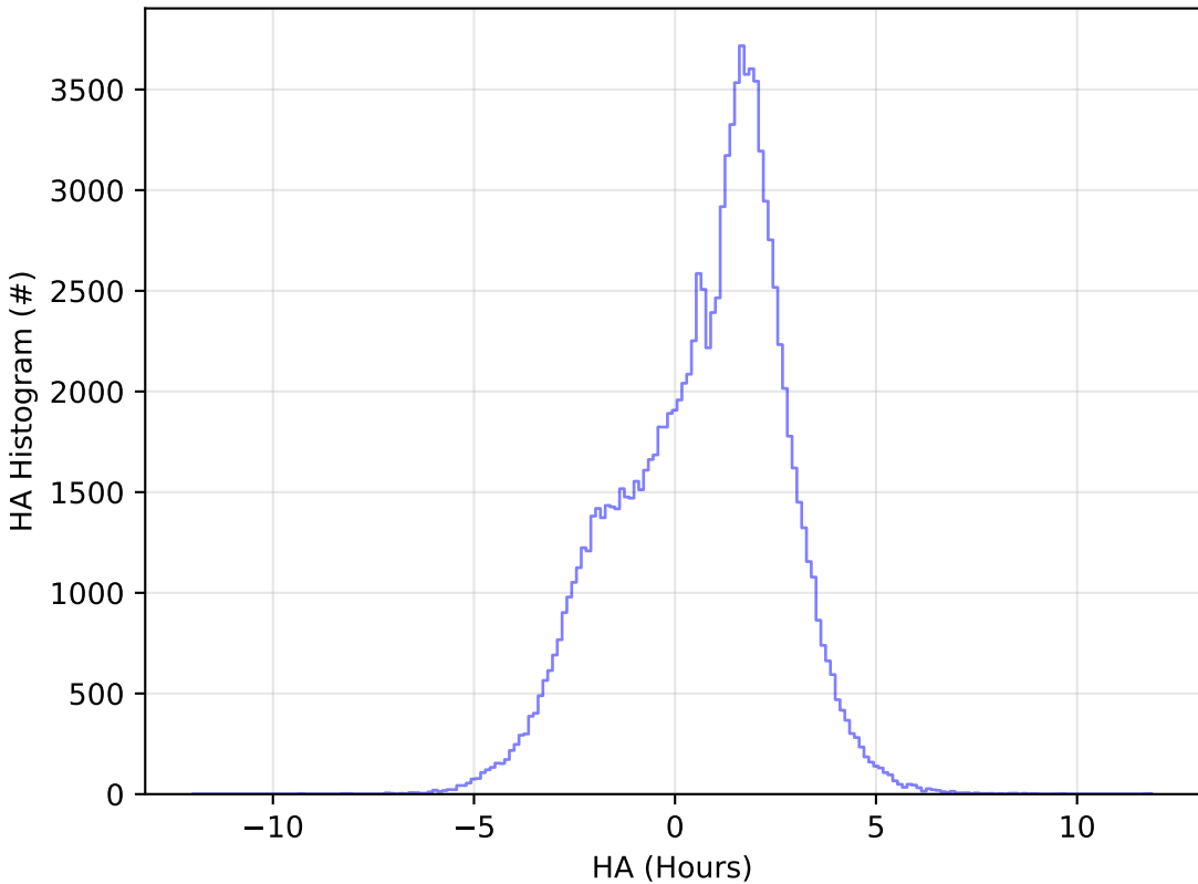
too_elab_r256_d3_griz_v3.4_10yrs All sky u band: HA Histogram
