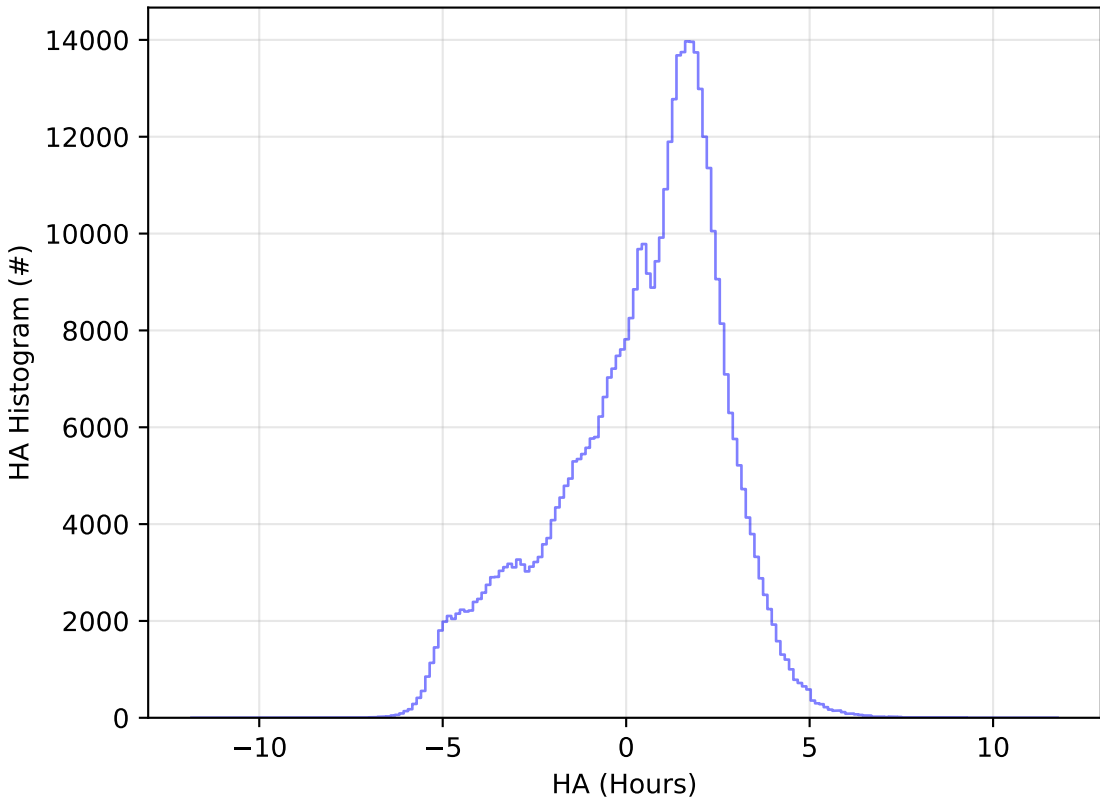
too_elab_r256_d3_griz_v3.4_10yrs All sky r band: HA Histogram
