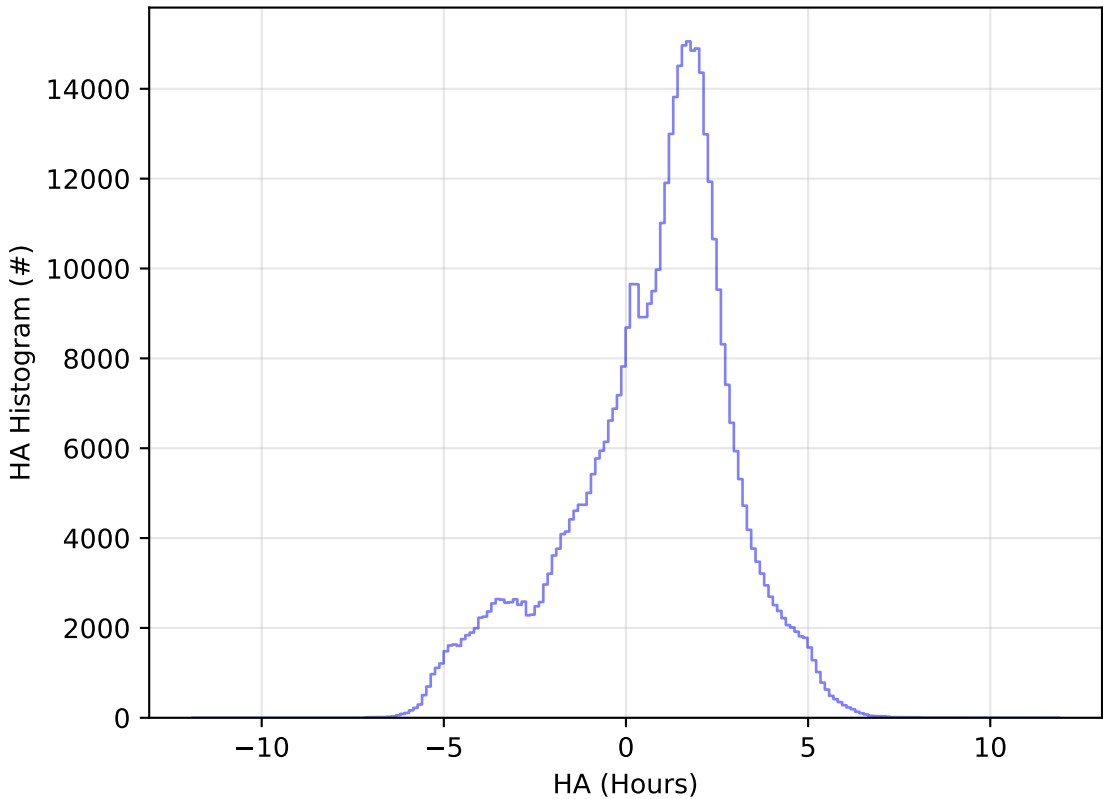
too_elab_r256_d3_griz_v3.4_10yrs All sky i band: HA Histogram
