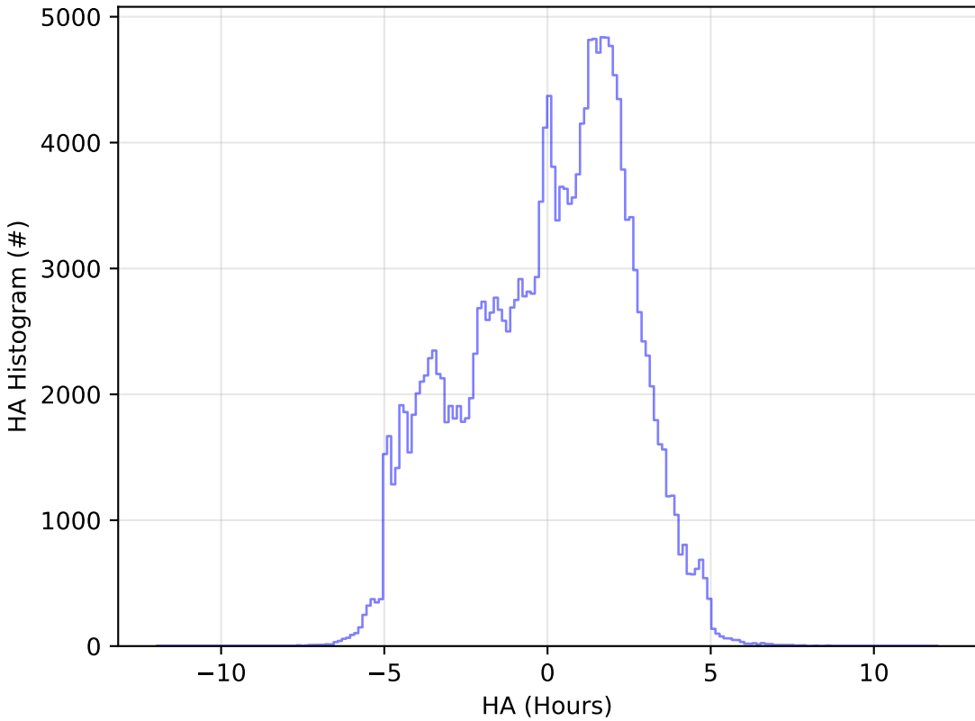
too_elab_r256_d3_griz_v3.4_10yrs All sky g band: HA Histogram
