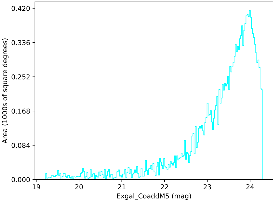
too_elab_r256_d3_griz_v3.4_10yrs Yr 3-4 u band: Exgal_CoaddM5
