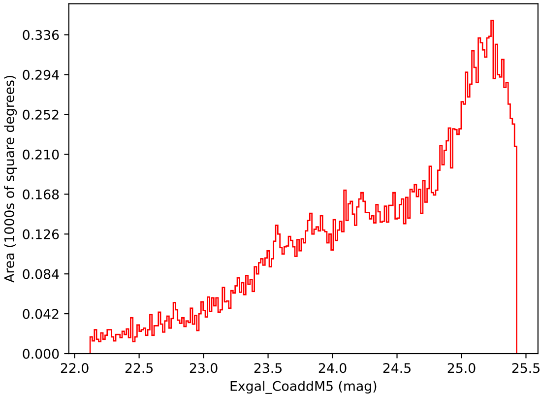
too_elab_r256_d3_griz_v3.4_10yrs Yr 3-4 i band: Exgal_CoaddM5
