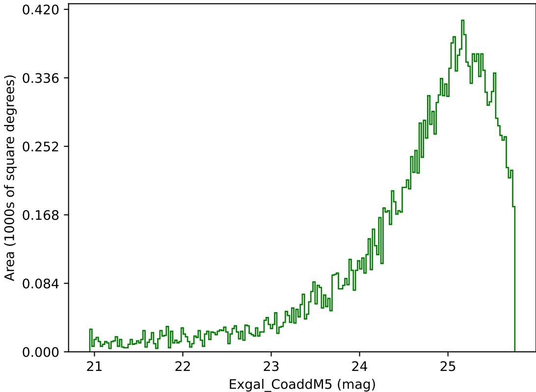
too_elab_r256_d3_griz_v3.4_10yrs Yr 3-4 g band: Exgal_CoaddM5
