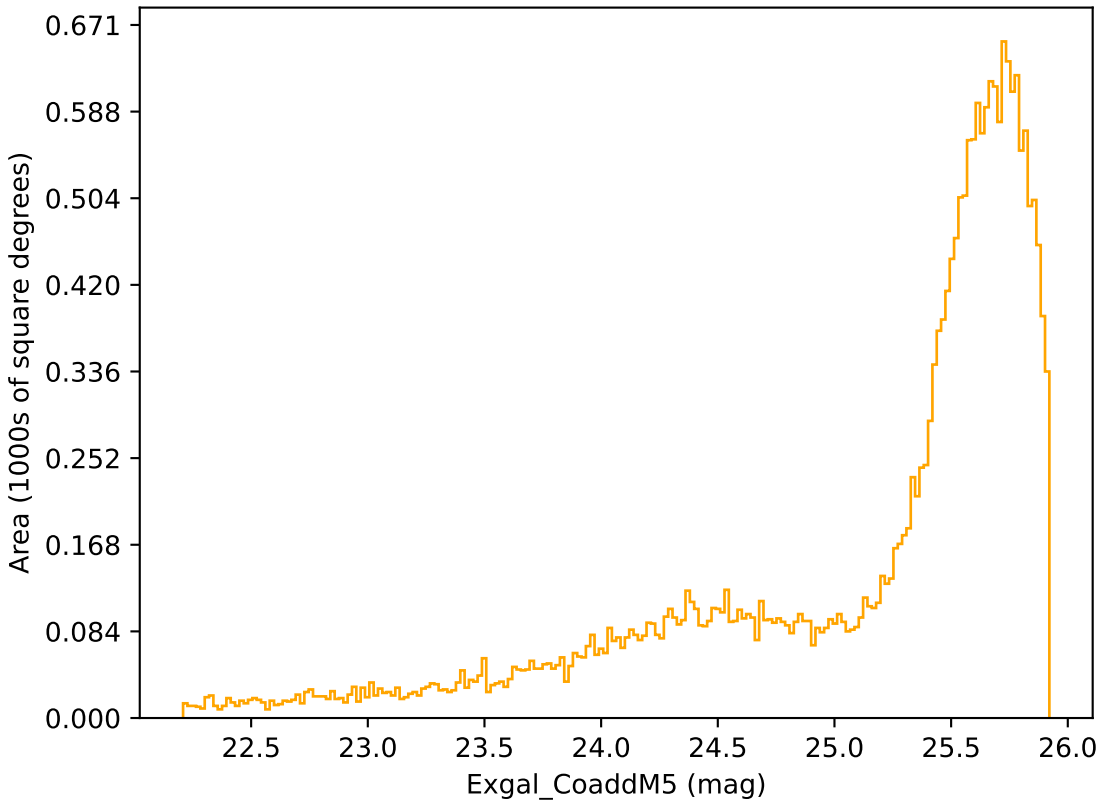
too_elab_r256_d3_griz_v3.4_10yrs Yr 1 r band: Exgal_CoaddM5
