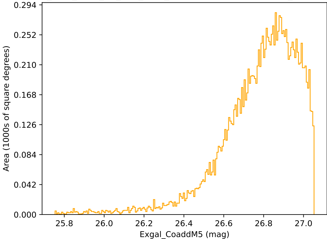
too_elab_r256_d3_griz_v3.4_10yrs WFD r band: Exgal_CoaddM5
