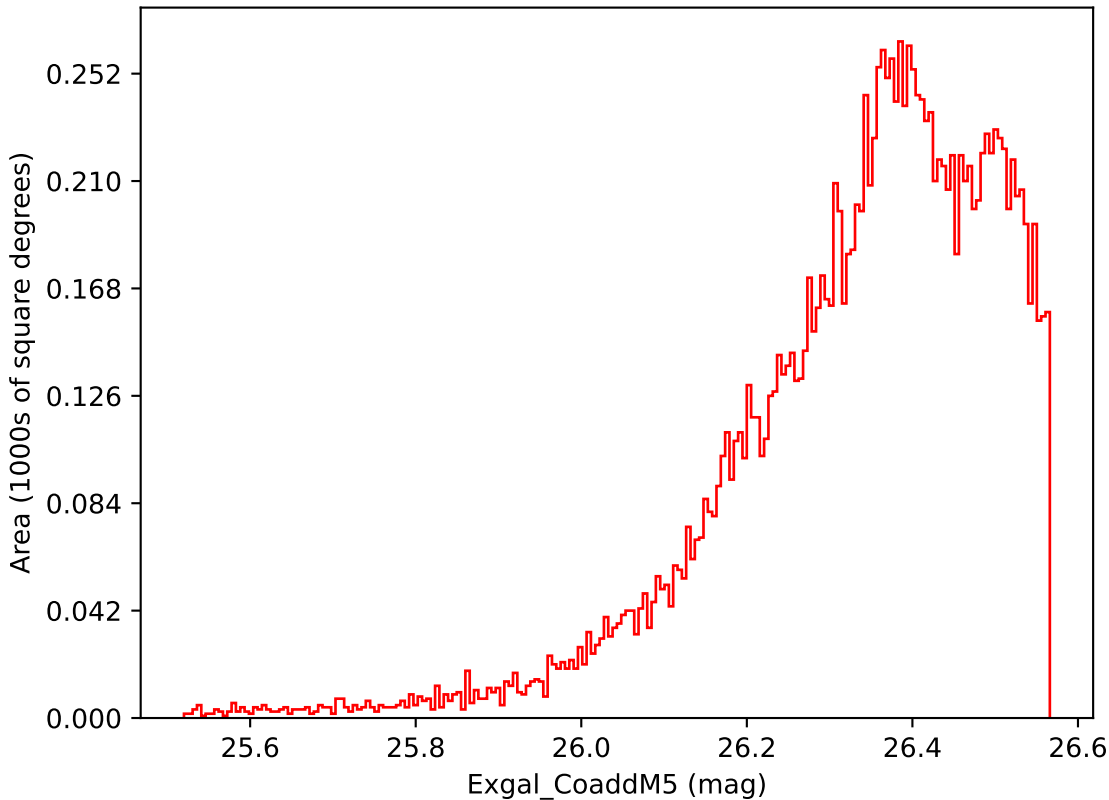
too_elab_r256_d3_griz_v3.4_10yrs WFD i band: Exgal_CoaddM5
