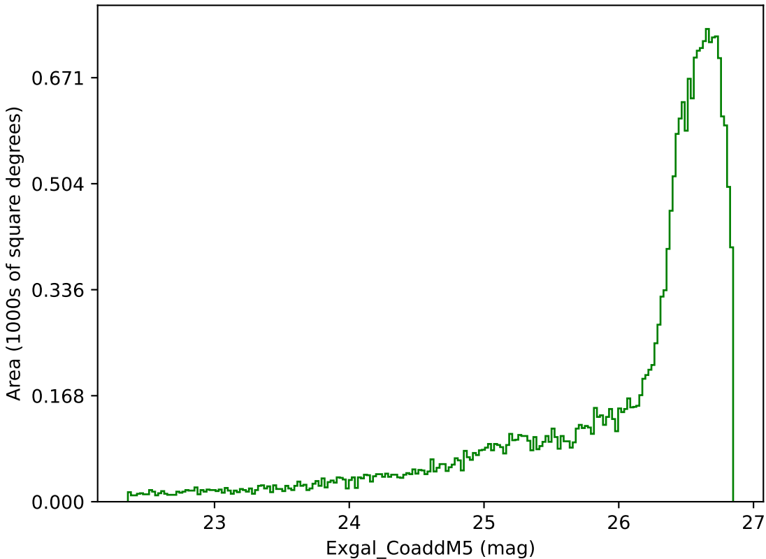
too_elab_r256_d3_griz_v3.4_10yrs All sky g band: Exgal_CoaddM5
