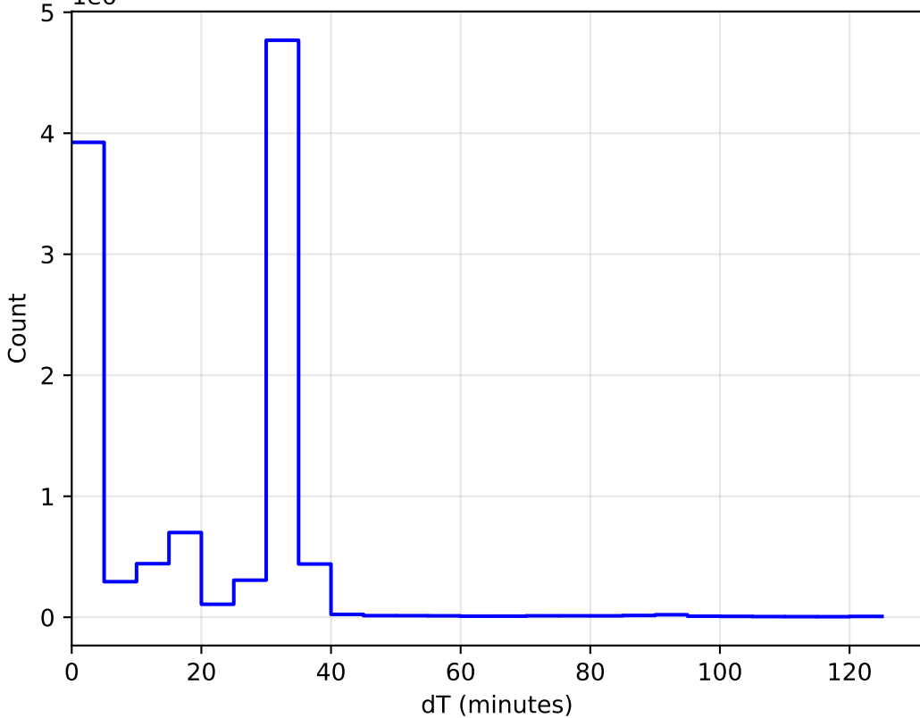
too_elab_r256_d3_griz_v3.4_10yrs WFD: DeltaT Histogram 1e6
