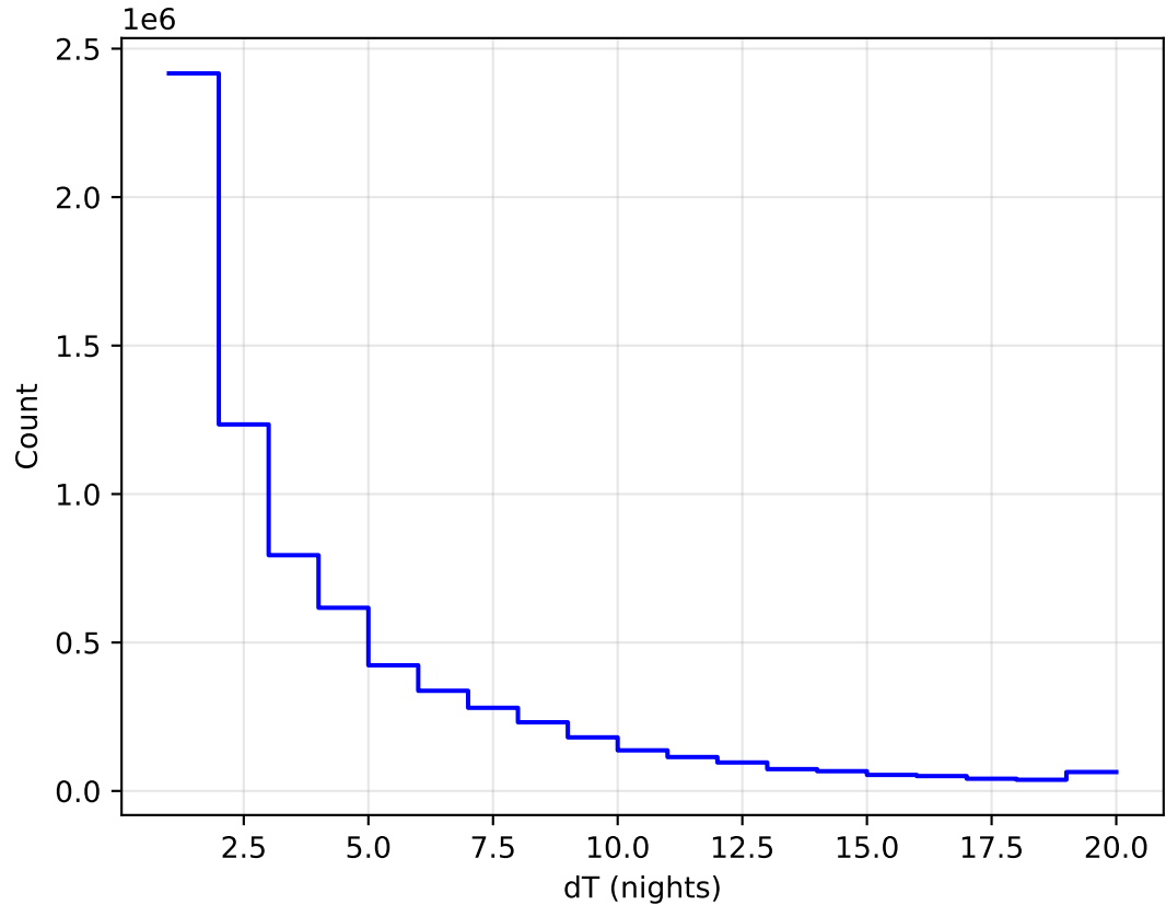
too_elab_r256_d3_griz_v3.4_10yrs WFD all bands: DeltaNight Histogram
