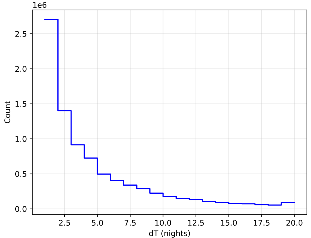
too_elab_r256_d3_griz_v3.4_10yrs All sky all bands: DeltaNight Histogram
