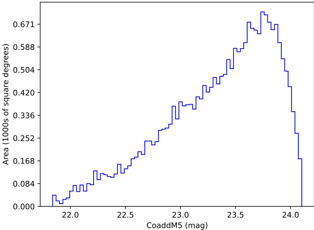
too_elab_r256_d3_griz_v3.4_10yrs Yr 3-4 y band: CoaddM5
