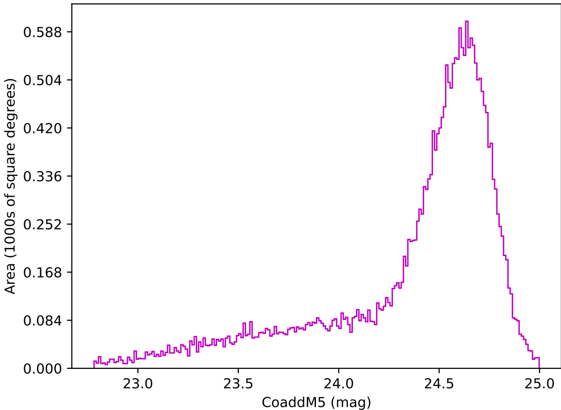
too_elab_r256_d3_griz_v3.4_10yrs Yr 1 z band: CoaddM5
