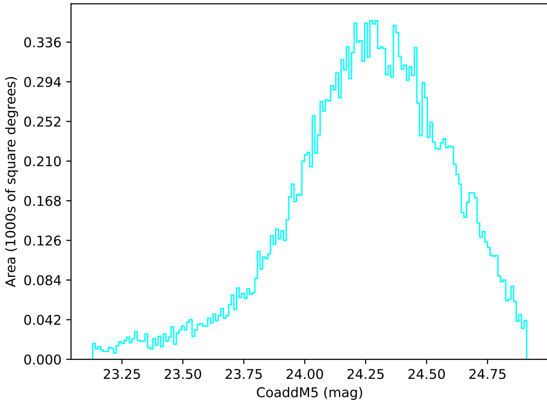
too_elab_r256_d3_griz_v3.4_10yrs Yr 1 u band: CoaddM5
