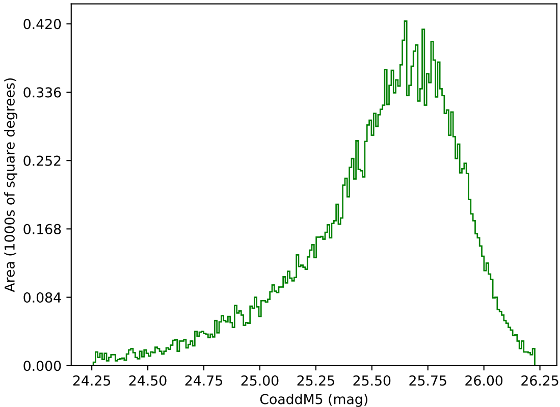
too_elab_r256_d3_griz_v3.4_10yrs Yr 1 g band: CoaddM5
