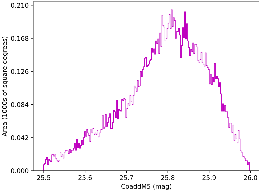
too_elab_r256_d3_griz_v3.4_10yrs WFD z band: CoaddM5
