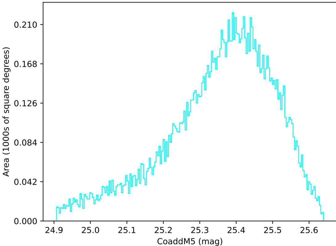
too_elab_r256_d3_griz_v3.4_10yrs WFD u band: CoaddM5
