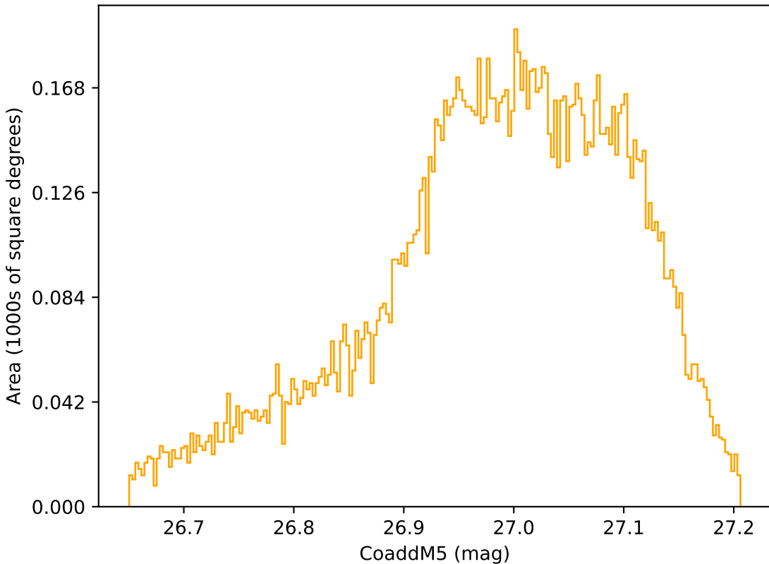
too_elab_r256_d3_griz_v3.4_10yrs WFD r band: CoaddM5
