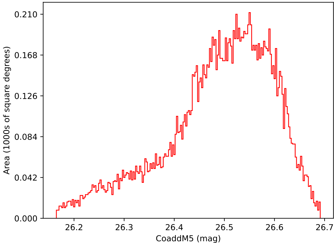
too_elab_r256_d3_griz_v3.4_10yrs WFD i band: CoaddM5
