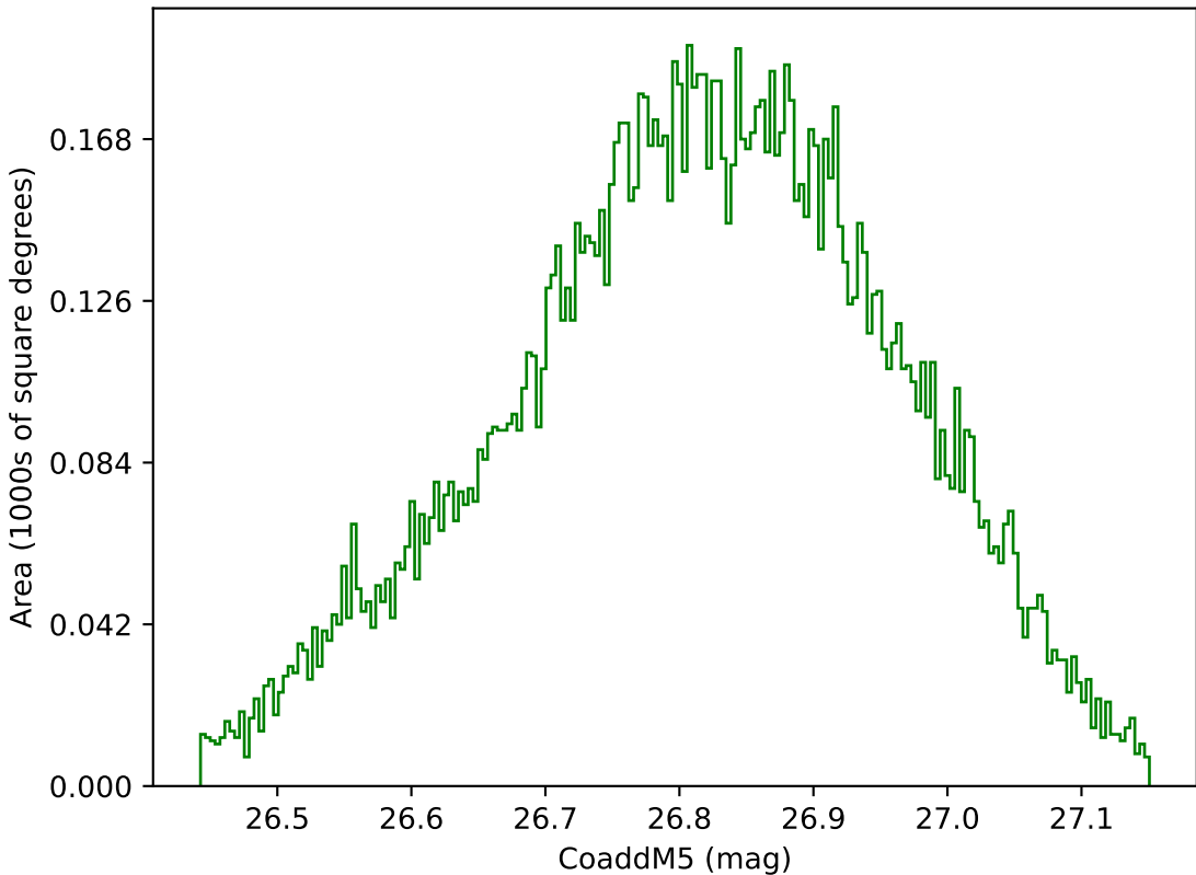
too_elab_r256_d3_griz_v3.4_10yrs WFD g band: CoaddM5
