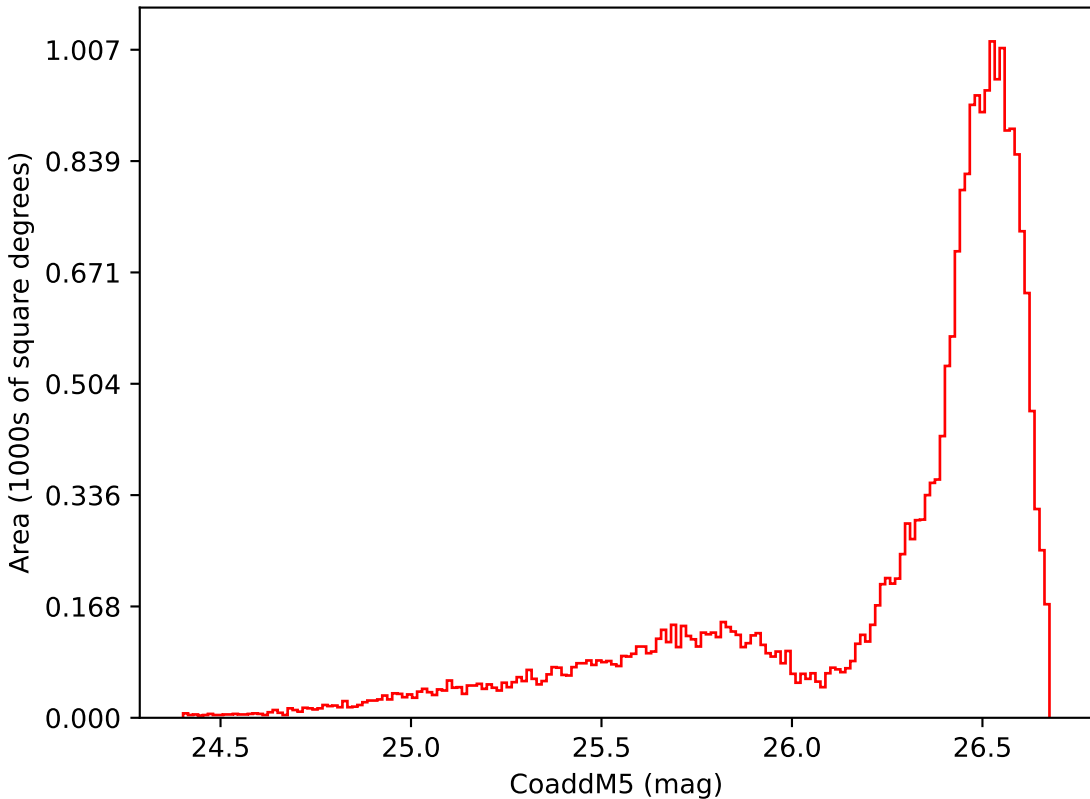
too_elab_r256_d3_griz_v3.4_10yrs All sky i band: CoaddM5
