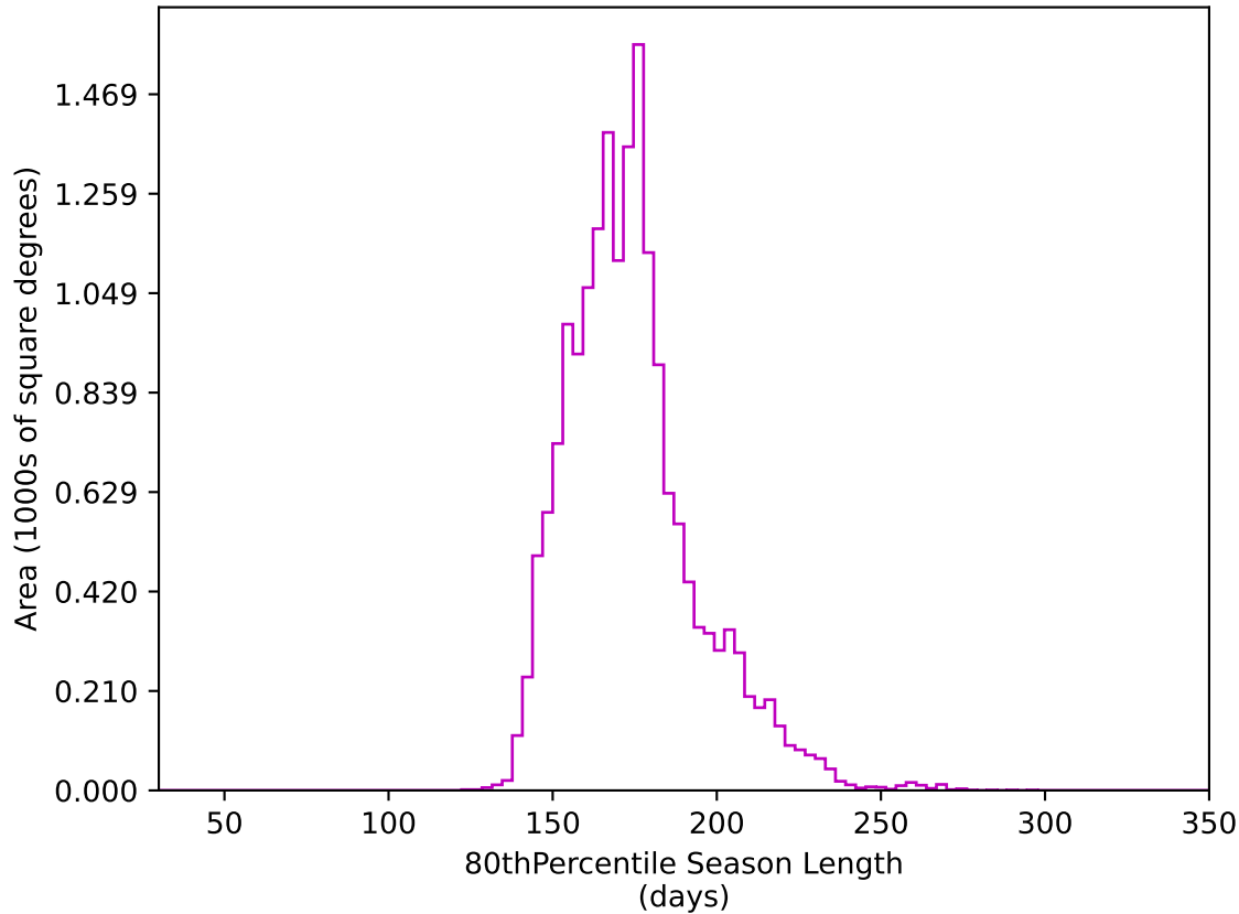
too_elab_r256_d3_griz_v3.4_10yrs WFD z band: 80thPercentile Season Length
