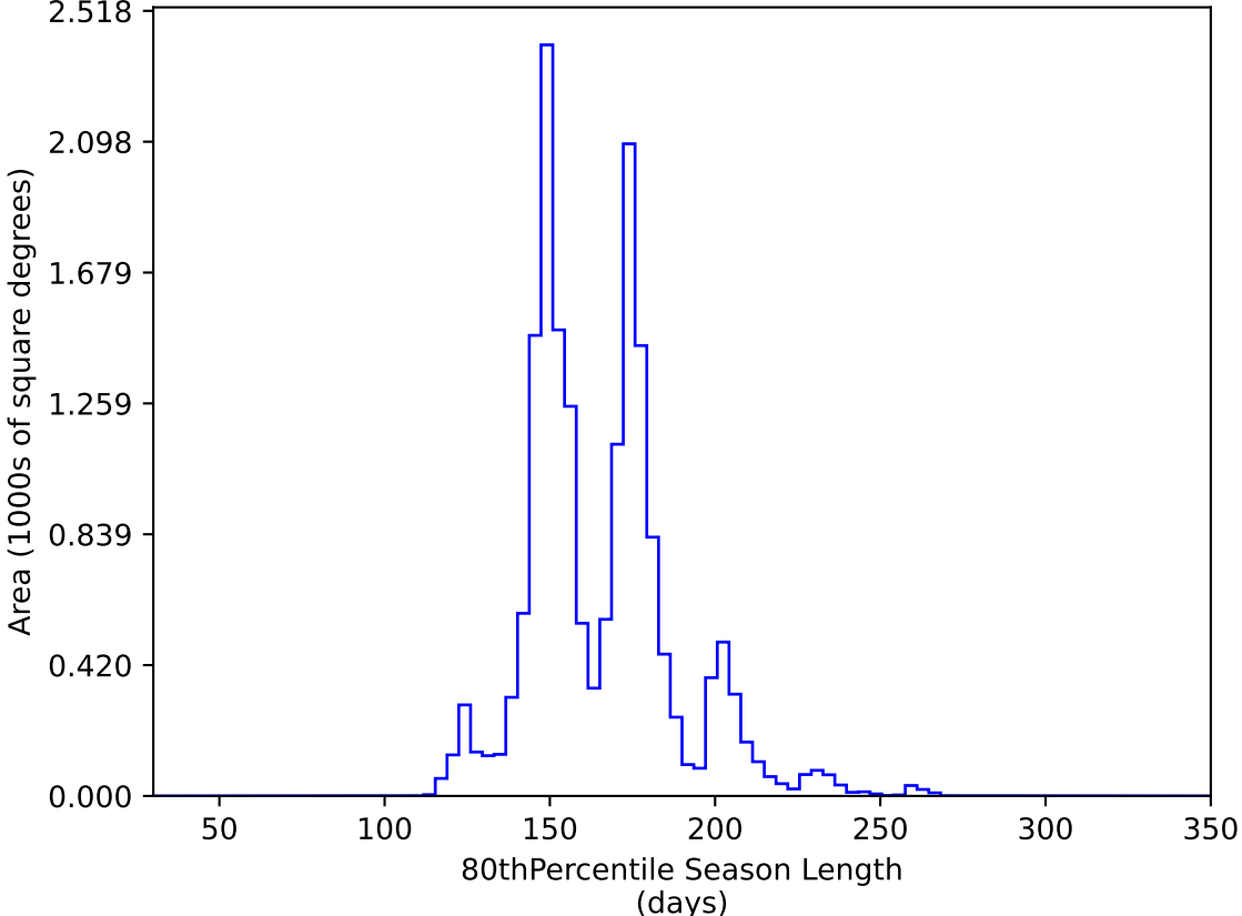
too_elab_r256_d3_griz_v3.4_10yrs WFD y band: 80thPercentile Season Length
