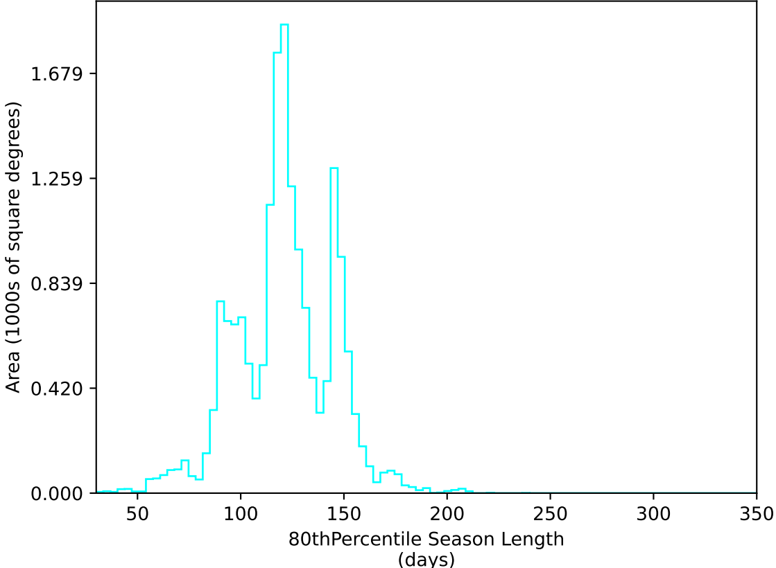
too_elab_r256_d3_griz_v3.4_10yrs WFD u band: 80thPercentile Season Length
