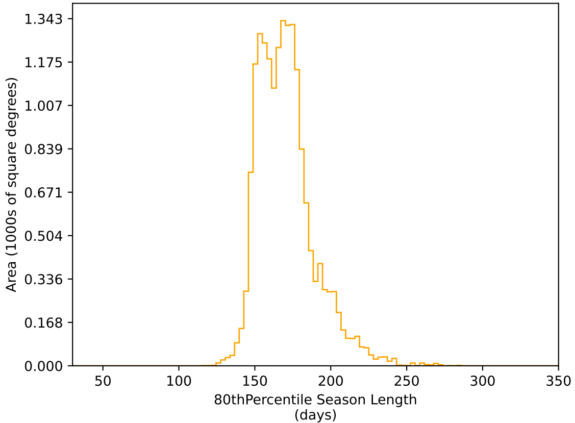
too_elab_r256_d3_griz_v3.4_10yrs WFD r band: 80thPercentile Season Length
