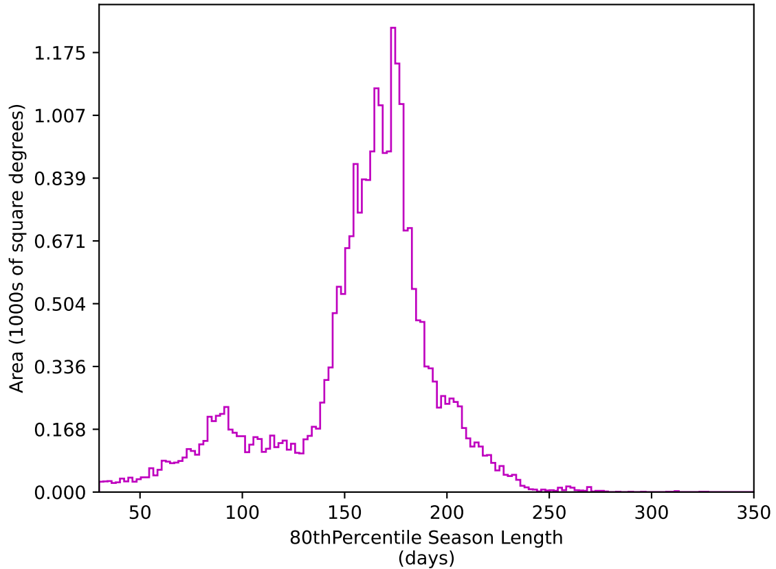
too_elab_r256_d3_griz_v3.4_10yrs All sky z band: 80thPercentile Season Length
