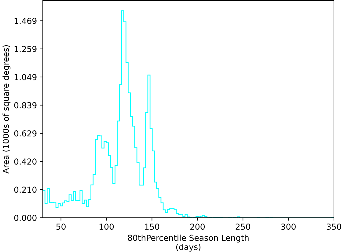
too_elab_r256_d3_griz_v3.4_10yrs All sky u band: 80thPercentile Season Length
