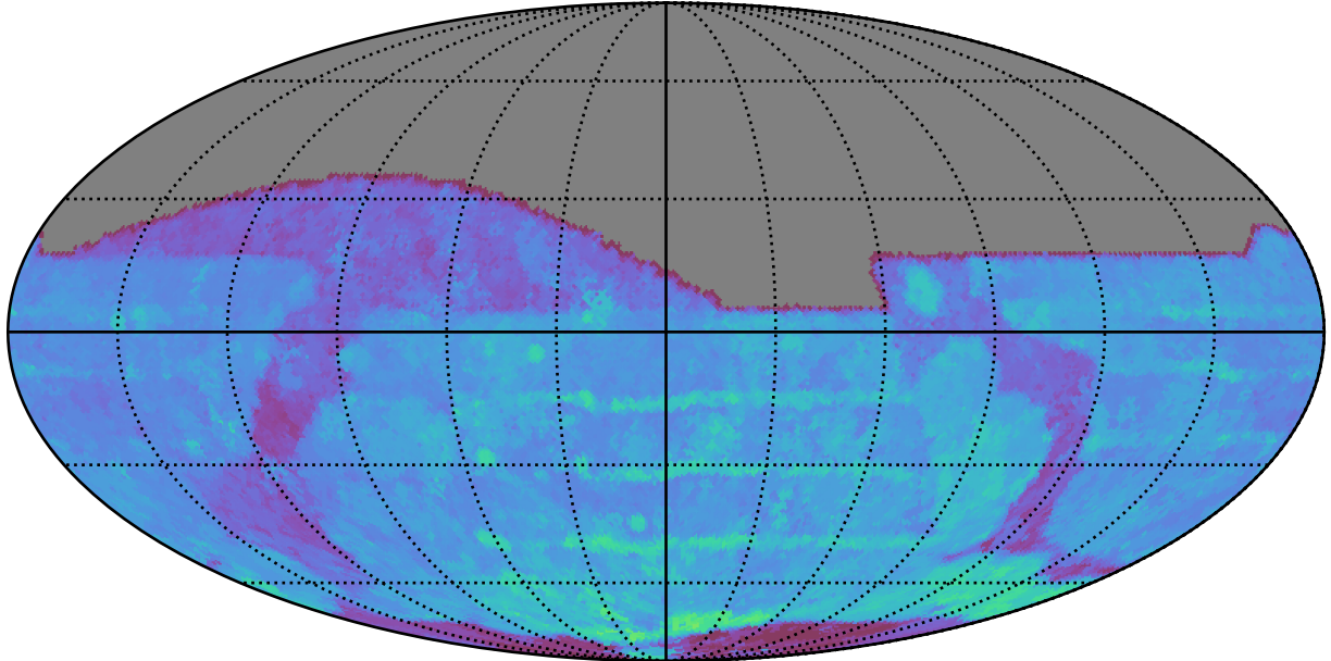
too_elab_r256_d3_griz_v3.4_10yrs All sky r band: 80thPercentile Season Length
