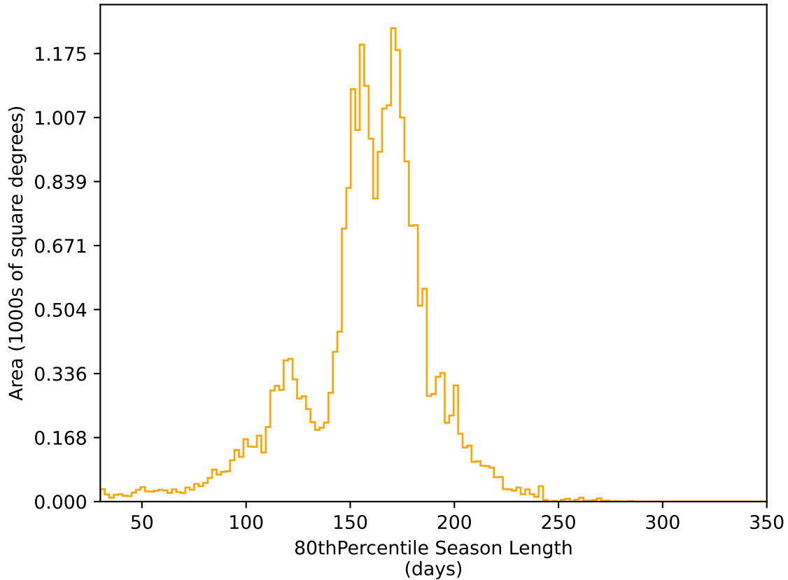
too_elab_r256_d3_griz_v3.4_10yrs All sky r band: 80thPercentile Season Length
