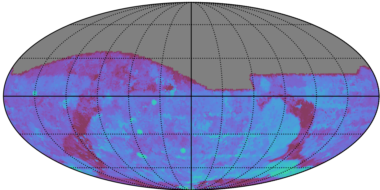
too_elab_r256_d3_griz_v3.4_10yrs All sky g band: 80thPercentile Season Length
