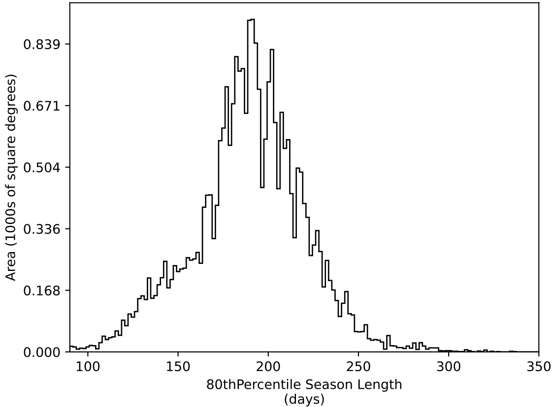
too_elab_r256_d3_griz_v3.4_10yrs All sky all bands: 80thPercentile Season Length
