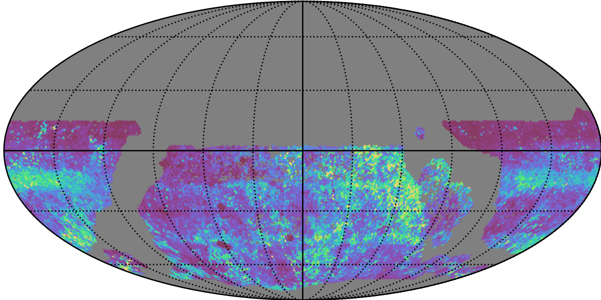
too_elab_r256_d3_griz_v3.4_10yrs WFD zy bands: 75th Percentile Intranight Timespan
